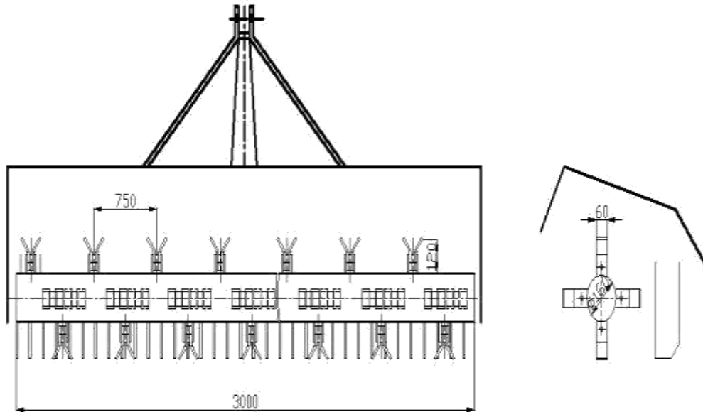
Figure 1. RT1 machine with “L” type knife.
