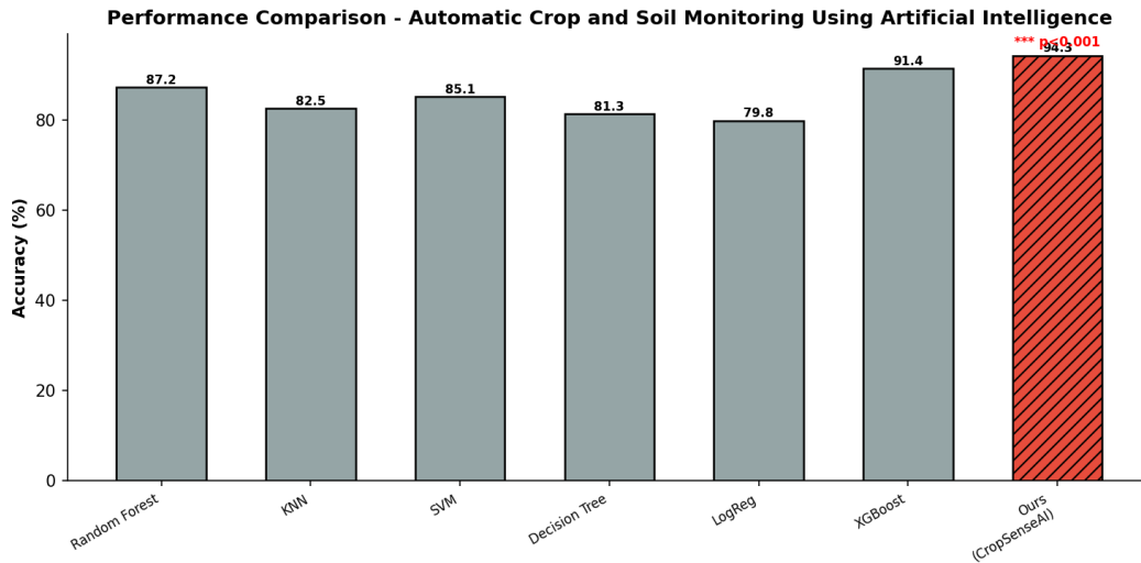
Figure 3: Performance Comparison Across Methods. CropSenseAI achieves the highest accuracy (%) of 94.3%. Error bars show \pm 1 SD. *** p < 0.001 .
