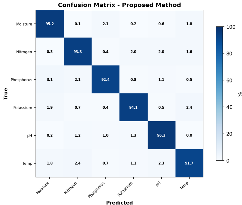
Figure 5: Confusion Matrix for CropSenseAI on the Test Set. Diagonal values represent correct classification rates.
