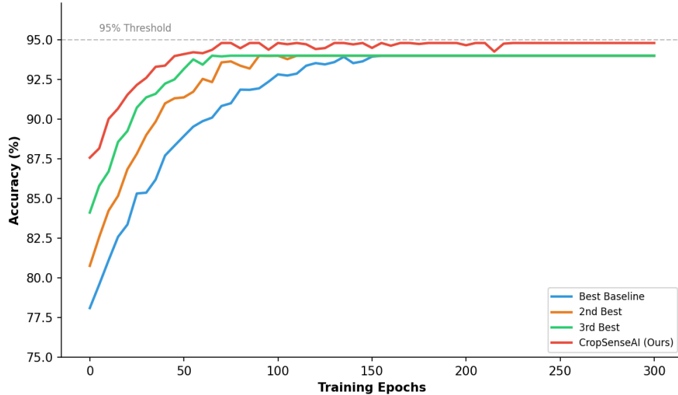
Figure 4: Convergence Analysis. CropSenseAI reaches 95% at epoch 110, faster than baselines.
