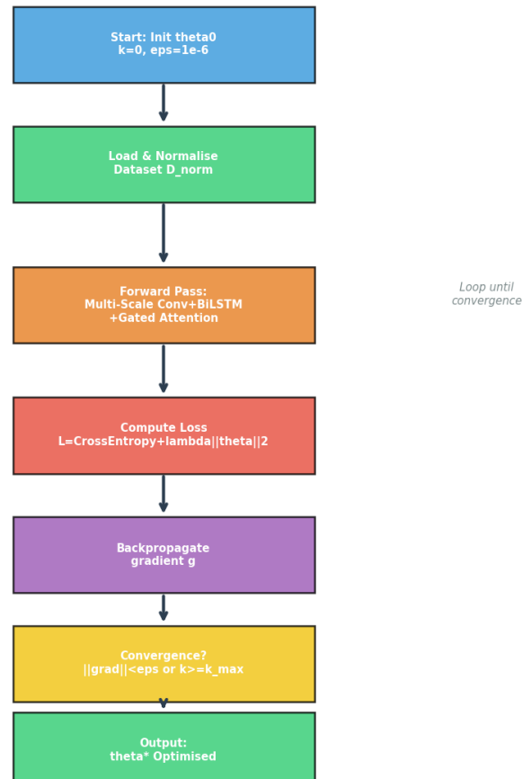
Figure 2: Algorithmic Flowchart of the CropSenseAI Training Procedure. Step numbers correspond to Algorithm 1.
