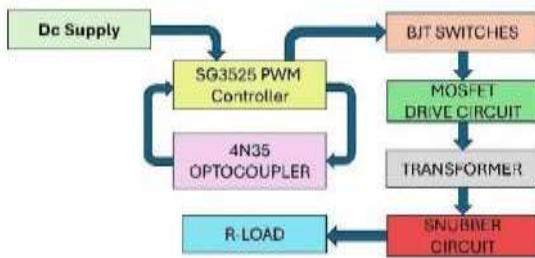
Fig.1. Block diagram of Third Harmonic Less Inverter.
