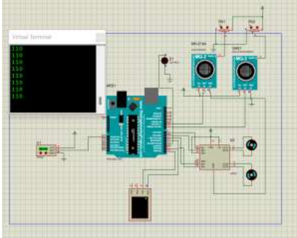
Fig. 11. Simulation Result
