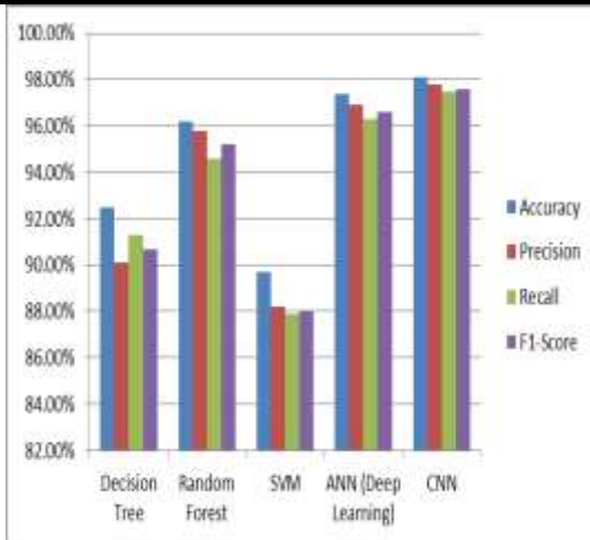
Figure 3: Comparison of Model Accuracy and Performance
