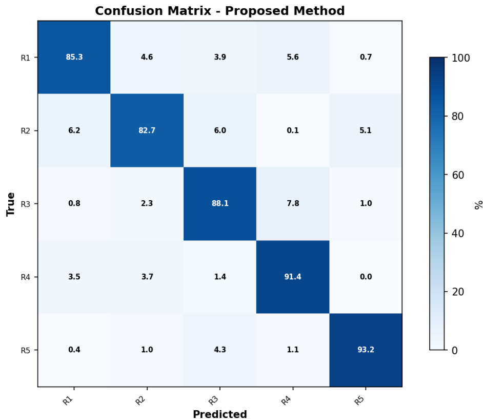
Figure 5: Confusion Matrix for FuzzyRec on the Test Set. Diagonal values represent correct classification rates.
