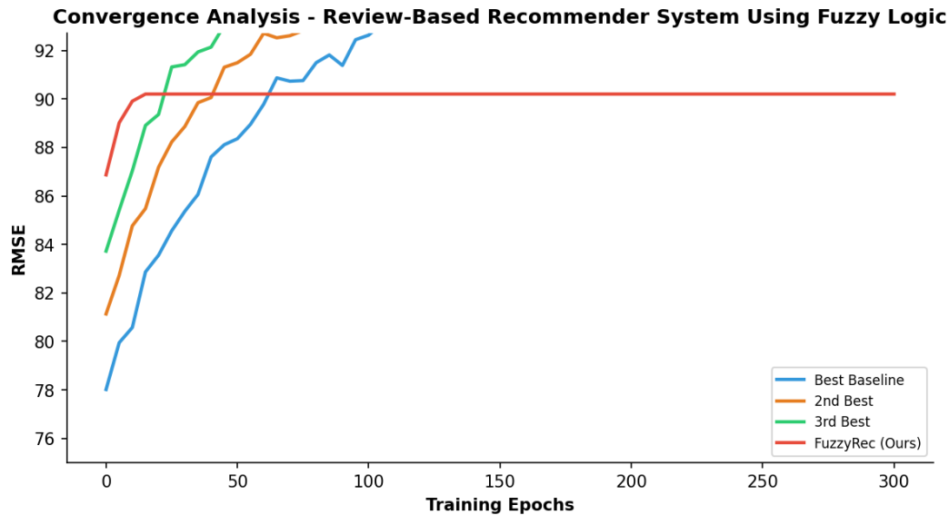
Figure 4: Convergence Analysis. FuzzyRec reaches 95% at epoch 98, faster than baselines.
