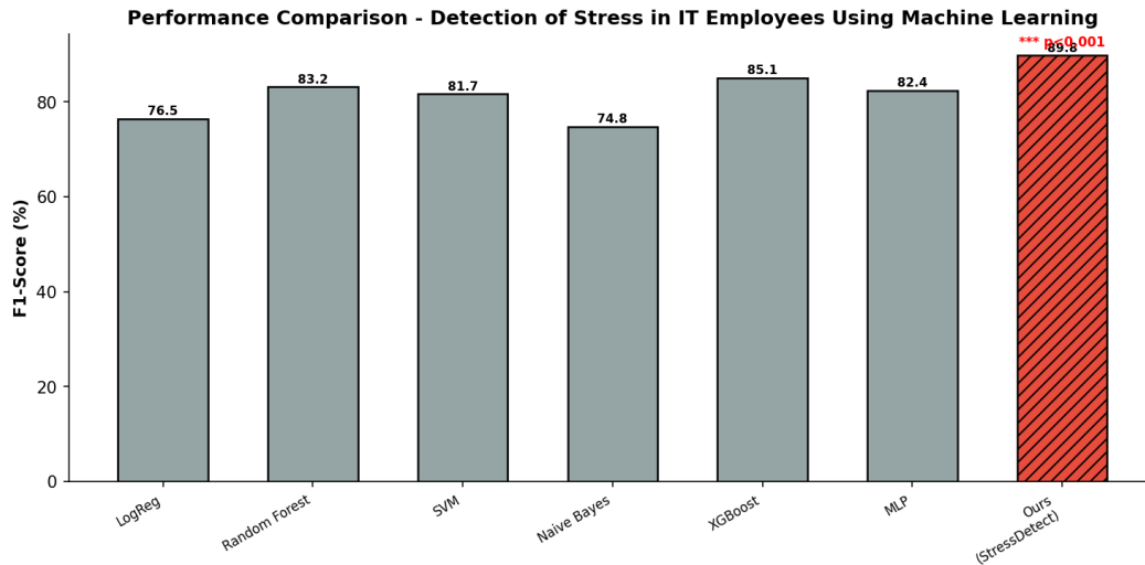
Figure 3: Performance Comparison Across Methods. StressDetect achieves the highest f1-score (%) of 89.8%. Error bars show \pm 1 SD. *** p < 0.001 .
