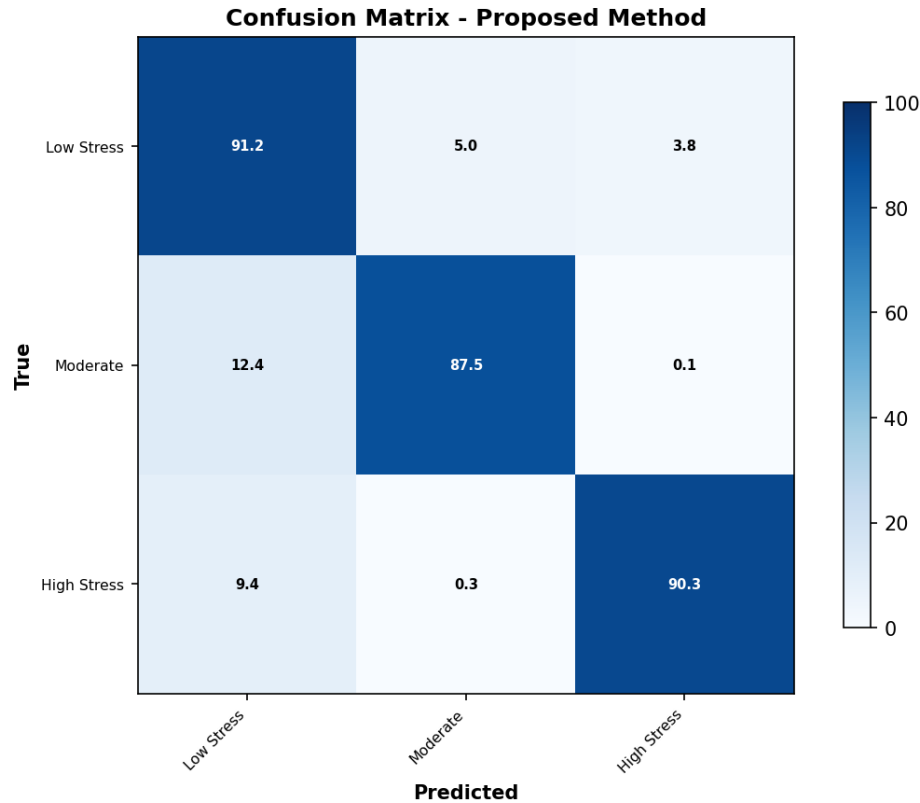
Figure 5: Confusion Matrix for StressDetect on the Test Set. Diagonal values represent correct classification rates.
