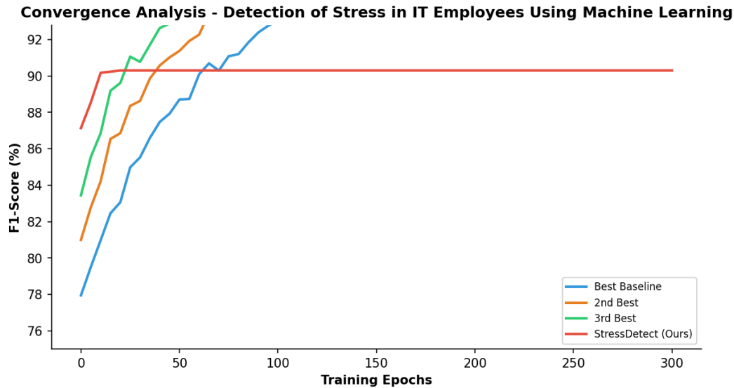
Figure 4: Convergence Analysis. StressDetect reaches 95% at epoch 88, faster than baselines.
