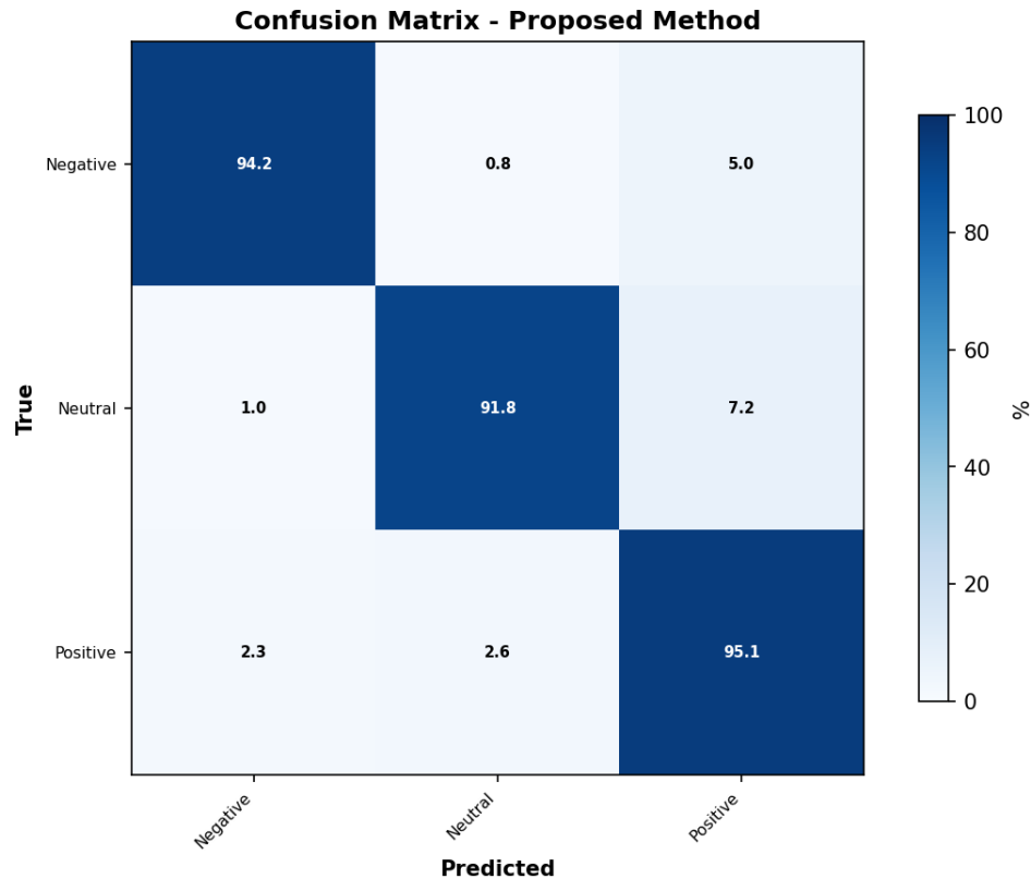
Figure 5: Confusion Matrix for SentNLP on the Test Set. Diagonal values represent correct classification rates.
