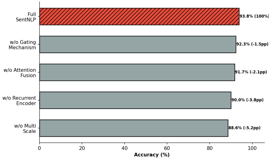
Figure 6: Ablation Study - Component Contribution. The recurrent encoder provides the largest single contribution.
