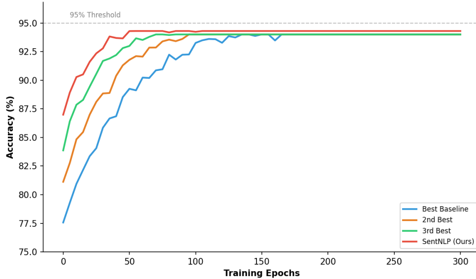
Figure 4: Convergence Analysis. SentNLP reaches 95% at epoch 62, faster than baselines.
