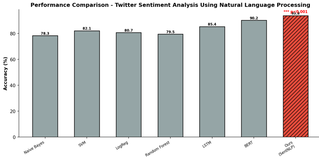
Figure 3: Performance Comparison Across Methods. SentNLP achieves the highest accuracy (%) of 93.8%. Error bars show \pm 1 SD. *** p < 0.001 .
