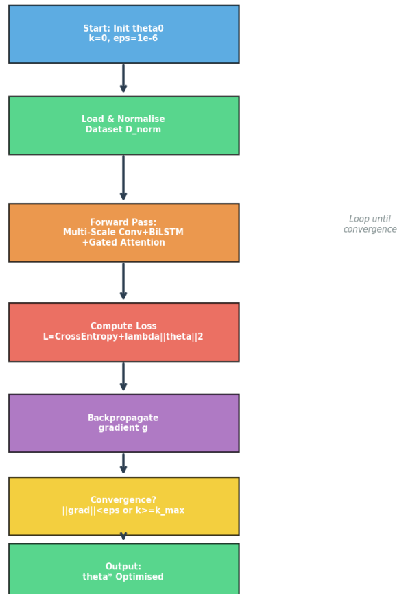
Figure 2: Algorithmic Flowchart of the WeapAlert Training Procedure. Step numbers correspond to Algorithm 1.
