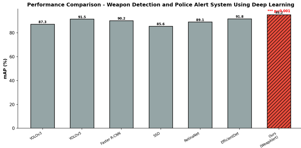
Figure 3: Performance Comparison Across Methods. WeapAlert achieves the highest map (%) of 95.2%. Error bars show \pm 1 SD. *** p < 0.001 .
