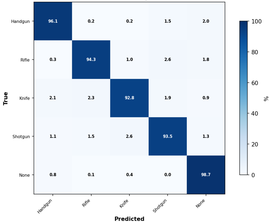
Figure 5: Confusion Matrix for WeapAlert on the Test Set. Diagonal values represent correct classification rates.
