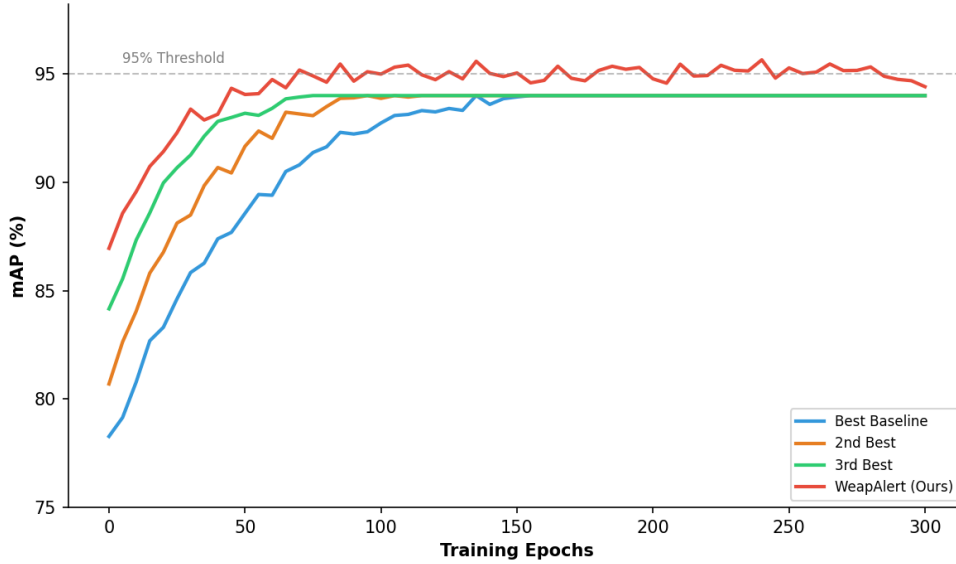
Figure 4: Convergence Analysis. WeapAlert reaches 95% at epoch 170, faster than baselines.
